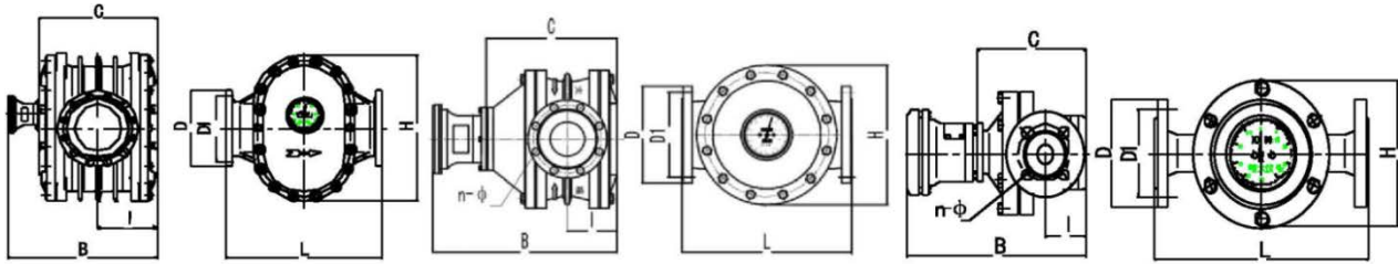
➤ LC-A Cast Iron Oval Gear Flow meter Dimensions (B=Register A dimensions) Unit :mm Table 3
